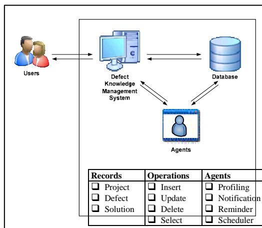
Figure 3: The proposed architecture of defect KMS
