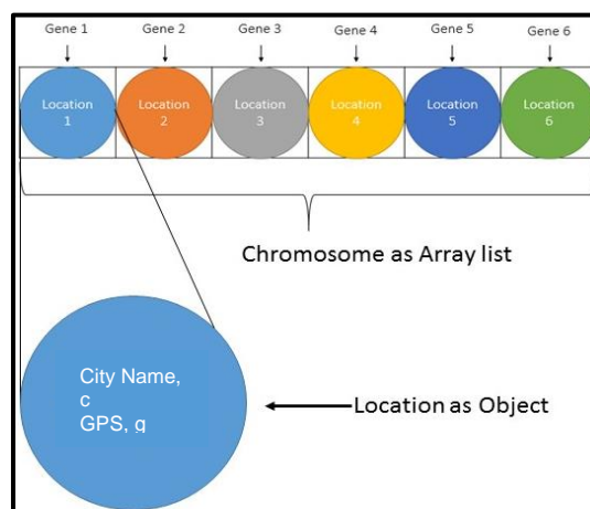
Figure 2. Chromosome Representation
