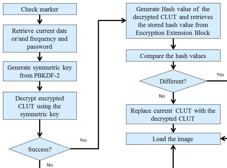
Figure 5. Process of Decryption/Viewing Image
