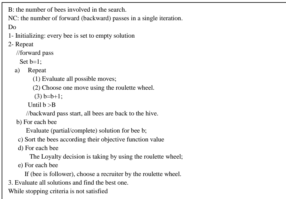
Figure 1. Steps of Bee Colony Optimization (Teodorvić, 2009)
