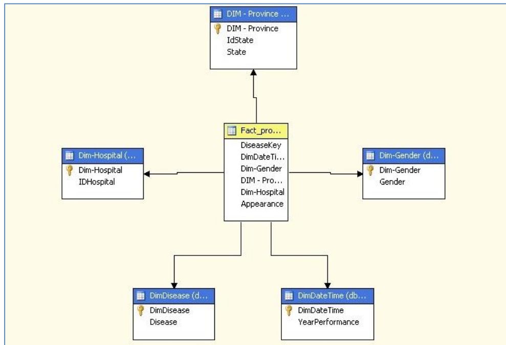
Figure 3. Star Schema Model of IIHS
