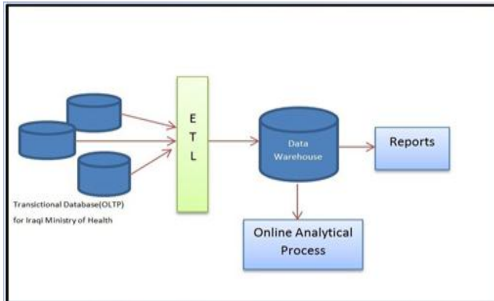
Figure 2. IIHS Architecture
